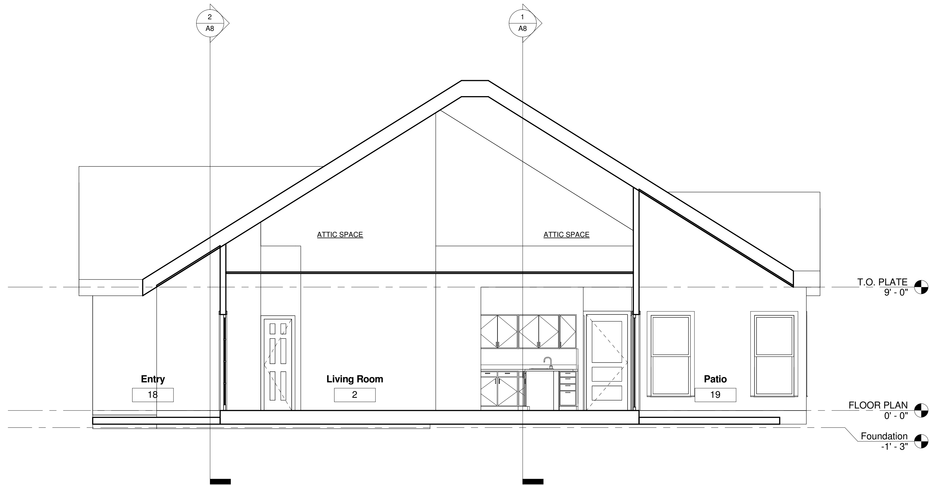
1 Section 1 1/4" = 1'-0"
