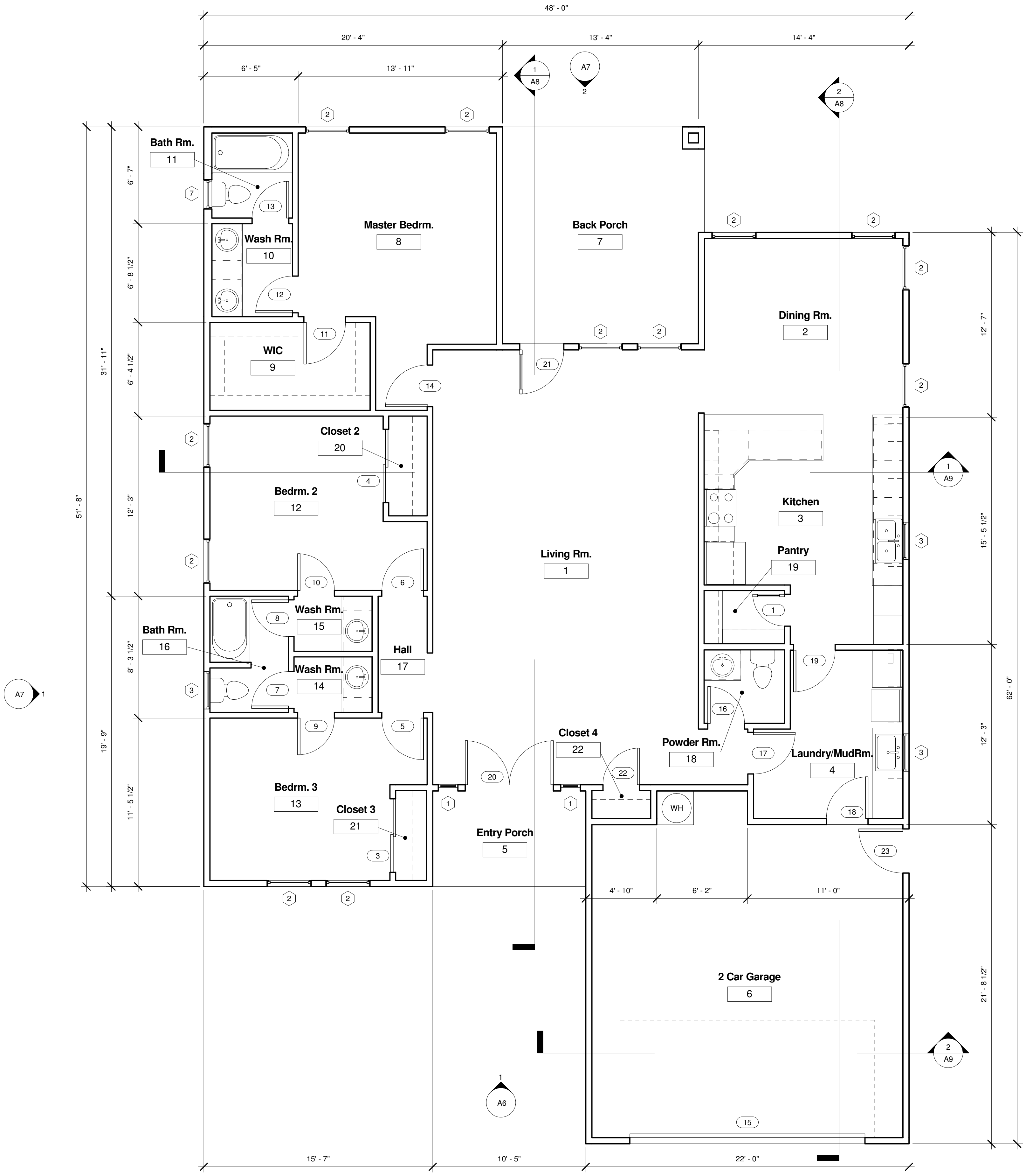
FLOOR PLAN 1/4" = 1'-0"
